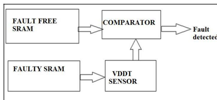
Figure 5: Block diagram of built in self-test architecture (BIST).
