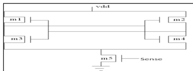
Figure 4: Sense amplifier.
