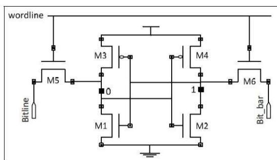
Figure 1: Existing 6T SRAM cell.
