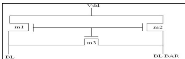
Figure 3: Precharge circuit.
